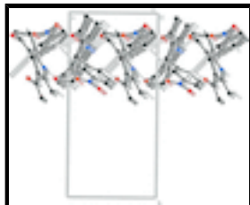
Fig. 2. Part of the crystal packing, showing the two-dimensional (010) layer. The weak hydrogen bonds and C—H... \pi interactions are shown as dashed lines. For the sake of clarity, the H atoms and disordered atoms not involved in the hydrogen-bonds pattern have been omitted.
