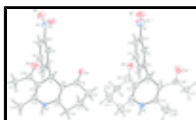
Fig. 1. The title molecule with the atom-numbering scheme, showing both the major (left) and minor (right) components. The displacement ellipsoids are drawn at the 30% probability level.
